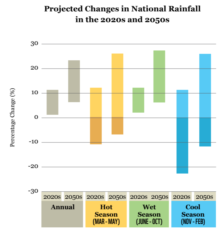
Figure 5.2. Range of average annual rainfall percentage change (low estimate to high estimate) relative to the 1980–2005 base period.
